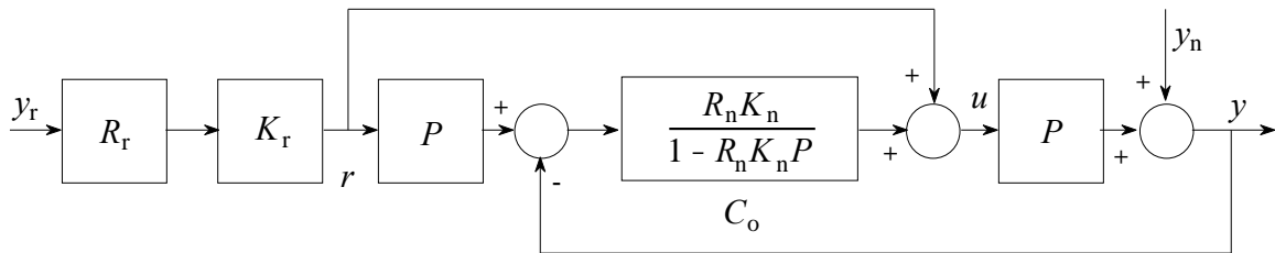
Fig. 5. The generic 2DF (G2DF) control system
