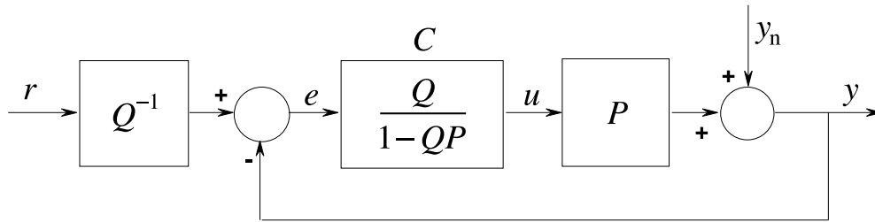
Fig. 2. The modified control system with an ARS regulator opening the closed-loop
