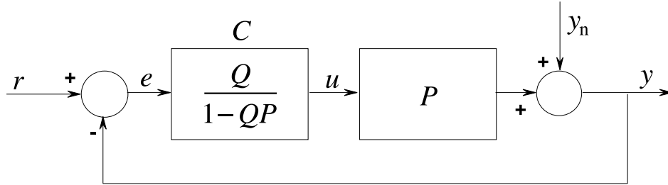
Fig. 1. Closed-loop with an ARS regulator
